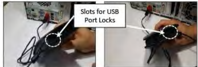
9 Identify slots for USB Port Locks on both side of hub
